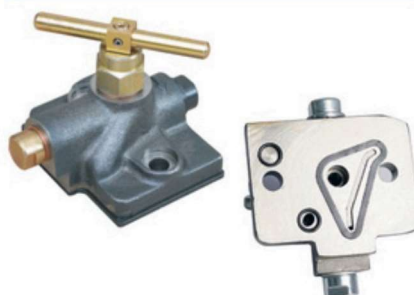
SrNo.:4196-B:TRANSPORT LOCK VALVE ASSLY. TAFE ALL NEW MODEL Ref. No.:
